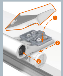
Insert caps.
