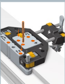
Drill holes in frame and door. Note left or right-hand doors.
